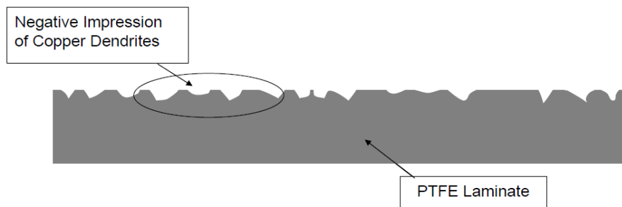
Figure 3 – Illustration of PTFE surface remaining after copper removal/etching
