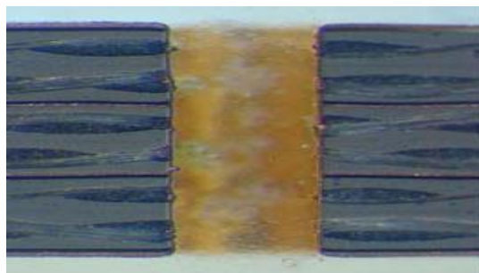
Figure 1 - Typical hole wall quality of RF-30A material
