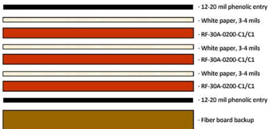
Figure 5 – Typical RF-30A rout stack-up
