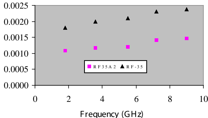
Dissipation Factor vs Frequency
