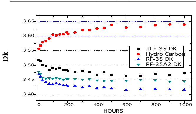
Dk Changes According to Aging Time (1,000 hrs.)
