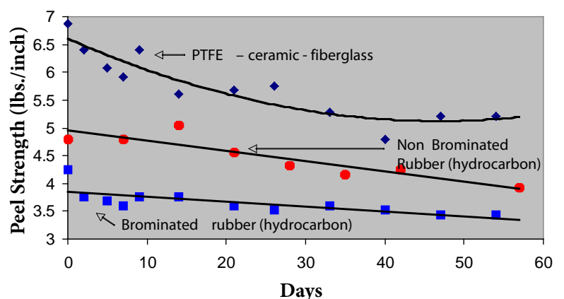
Copper Peel Strength Degradation (hold @ 150° C)
